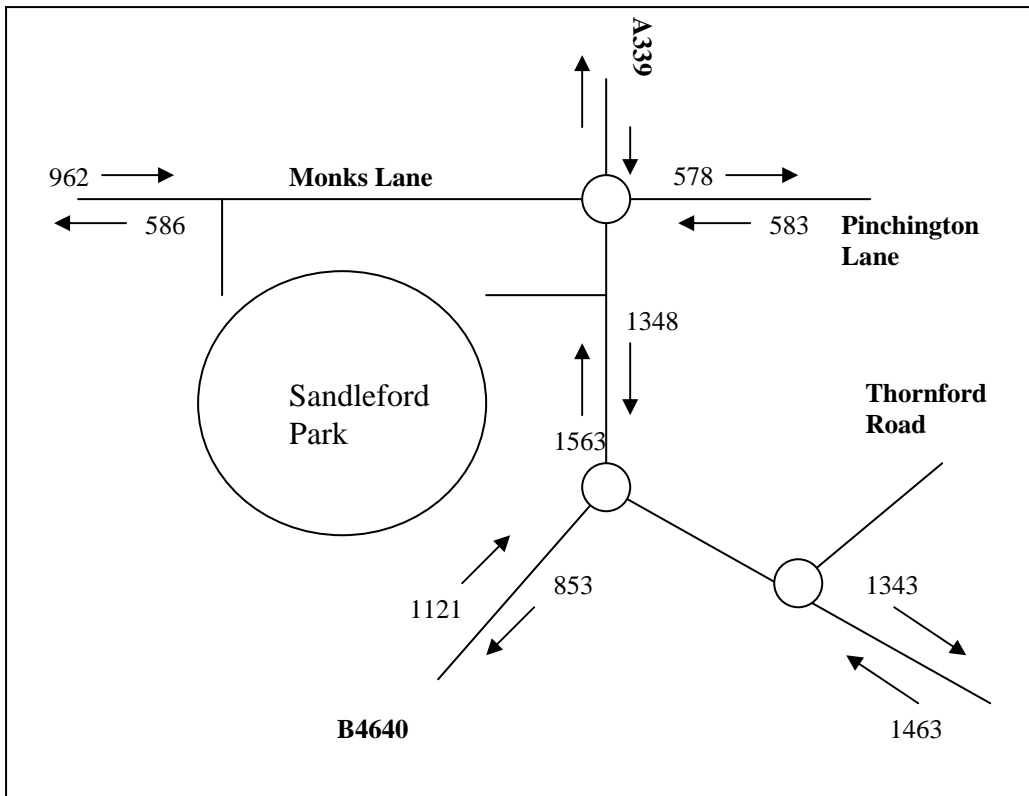
AM 2026 overall traffic flows
