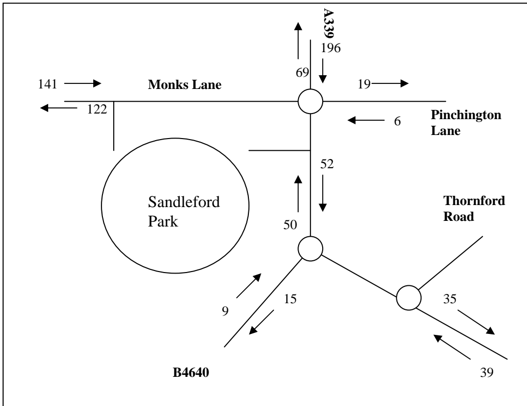
PM 2026 A339 Access
