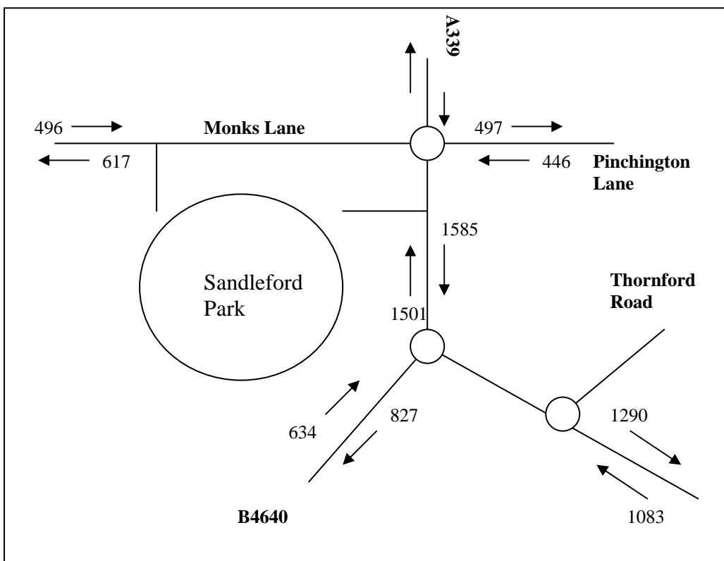
PM 2026 overall traffic flows
