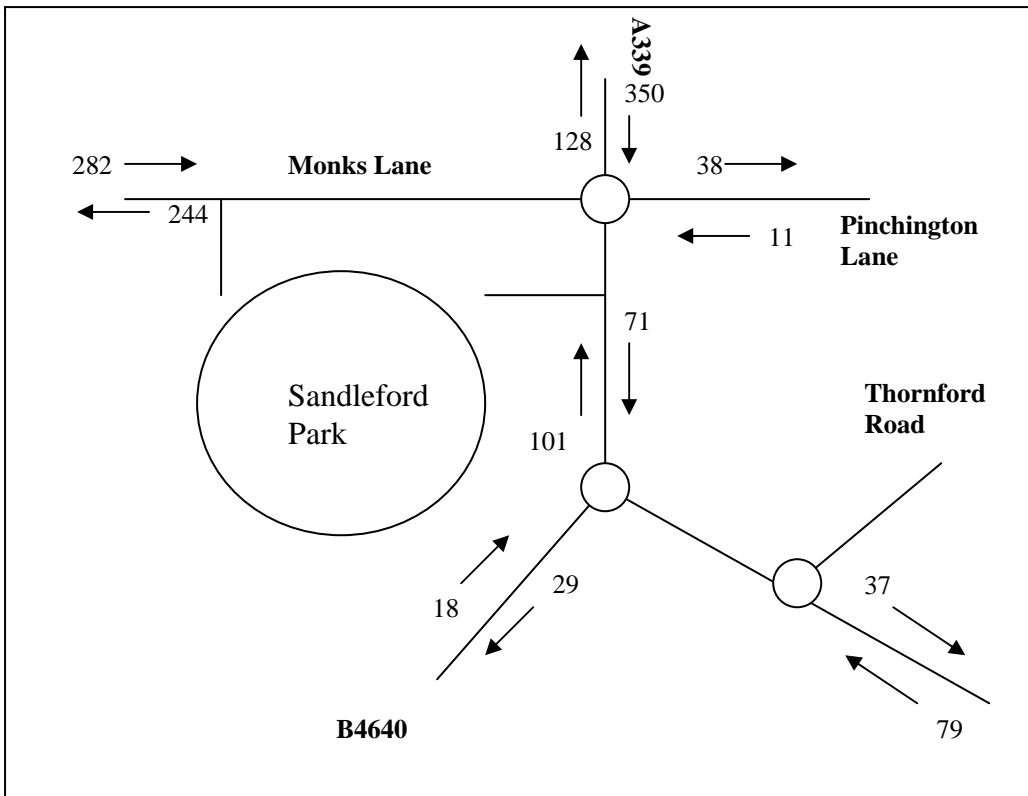
PM 2036 A339 Access
